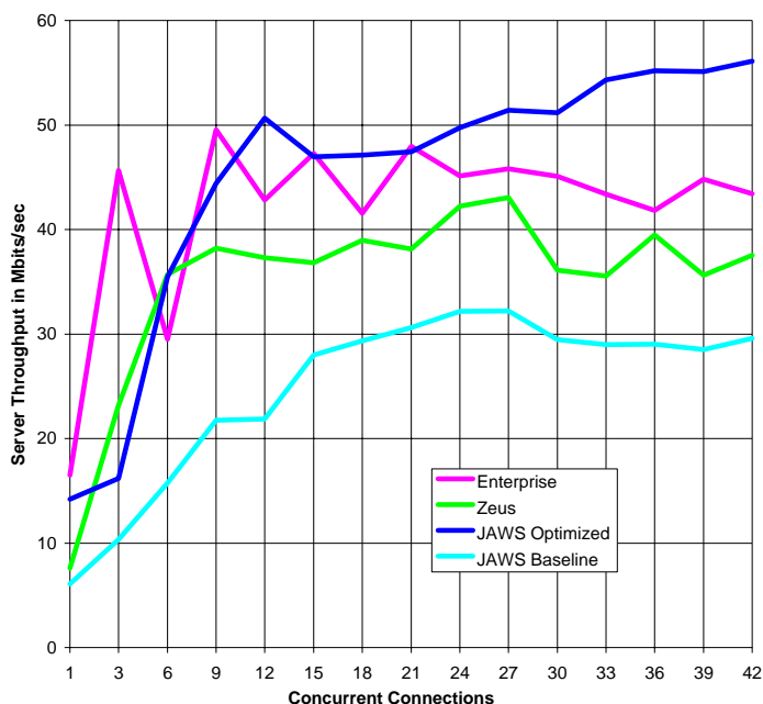
Figure 8: Comparative Performance for JAWS
