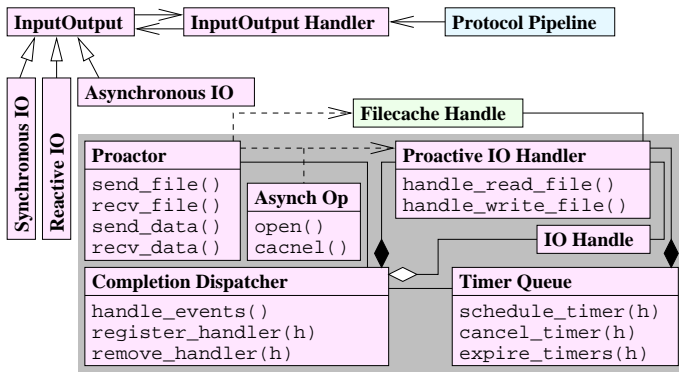
Figure 6: Structure of the Proactor Pattern in JAWS
