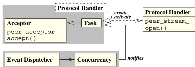
Figure 4: Structure of the Acceptor Pattern in JAWS
