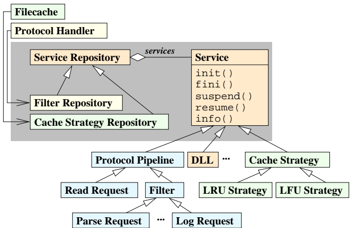
Figure 7: The Service Configurator Pattern in JAWS
